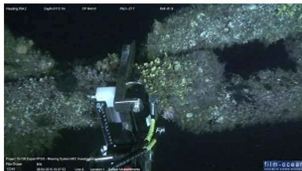
Example of bar diameter measuring tool in use on catenary chain
